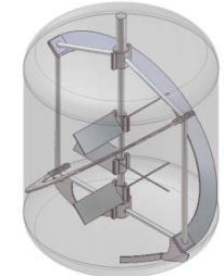
Coax Coaxial impeller
