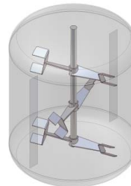
HPCFI High performance counter flow impeller
